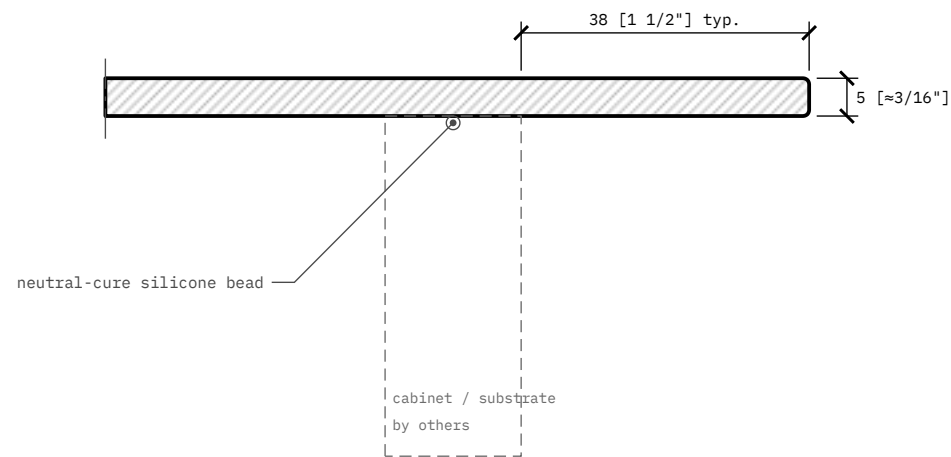
5 5 MM SOLID PLATE D01 SCALE 1:1 • 39.6 kg/m 2 • 8.1 lb/ft 2
